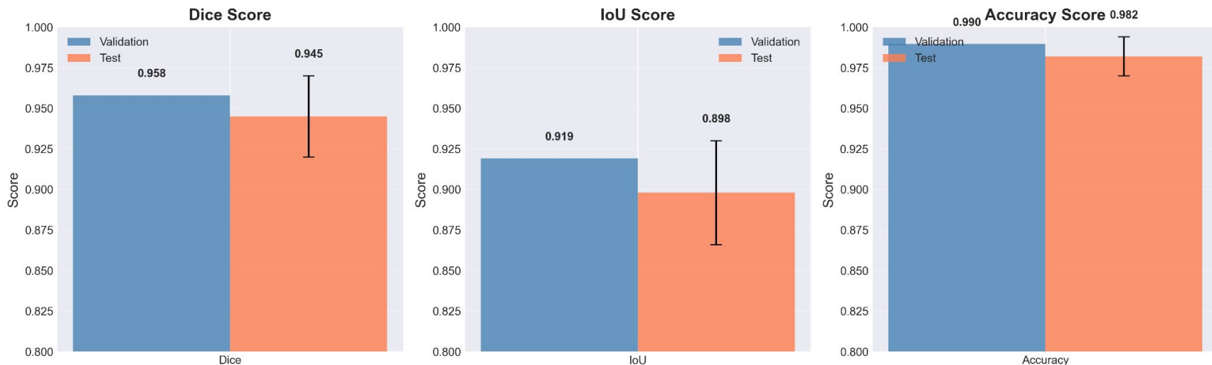
Validation vs Test Performance - unet_resnet34_spheroid
